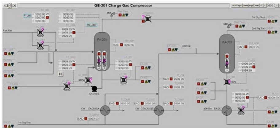
Figure 1. High-performance HMIs following ISA-101 use grayscale graphics and sparse color to draw attention to abnormal situations. Source: ISA/Maverick Technologies webinar, “ High Performance HMI Done Right ”
