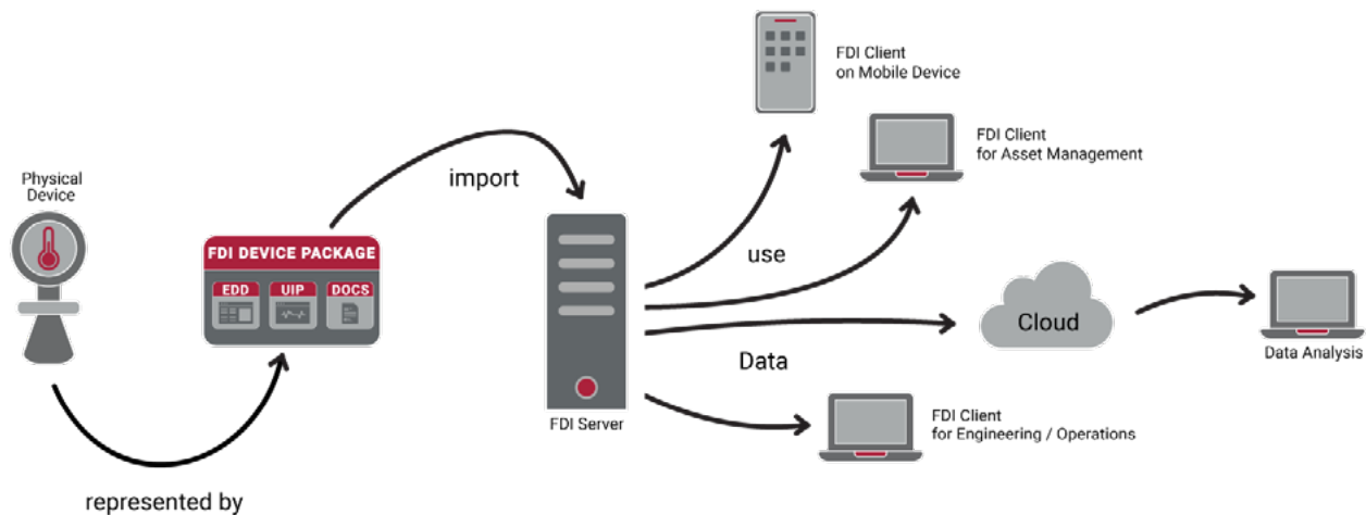
Figure 3: FDI supports communication with many different clients, including asset management systems, with compatibility assured by testing provided by the FieldComm Group.
