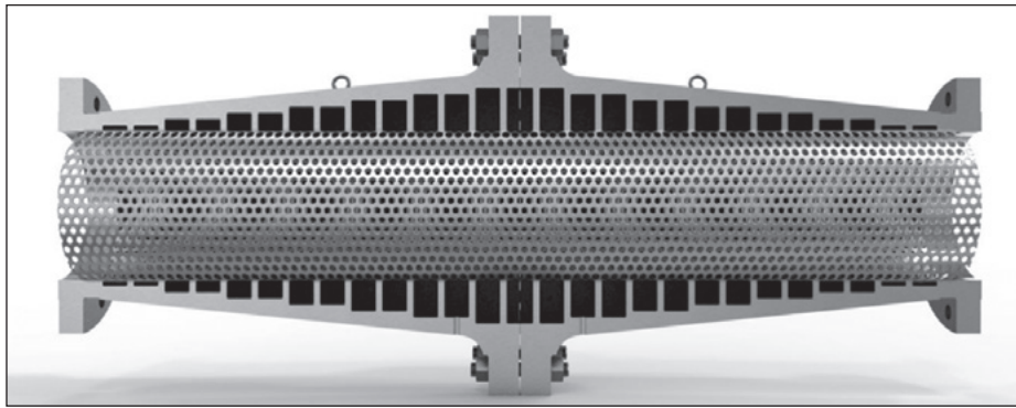
Figure 6. This modal suppressor employs a series of varying sized chambers to generate destructive interference over a range of frequencies, with virtually no pressure drop.
