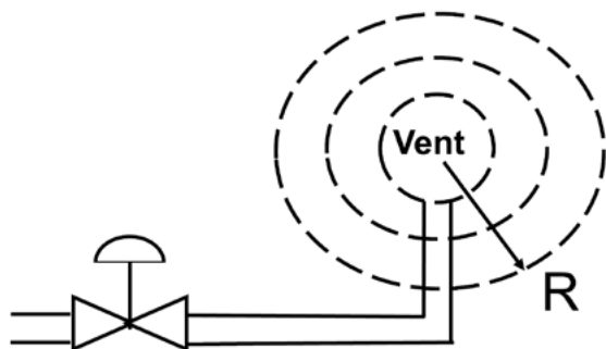
Figure 1. Noise point sources (top) lose sound energy quickly, falling with distance squared. Control valve noise (bottom) radiates sound from the pipe itself, as depicted in this piping cross section, so the sound levels drop much more slowly with distance.
