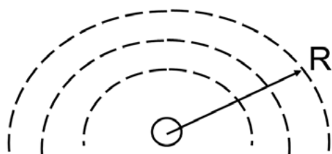
Figure 1. Noise point sources (top) lose sound energy quickly, falling with distance squared. Control valve noise (bottom) radiates sound from the pipe itself, as depicted in this piping cross section, so the sound levels drop much more slowly with distance.
