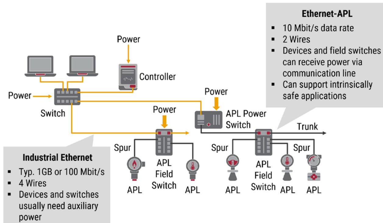
Figure 1: Ethernet-APL field devices will connect to Ethernet switches, which in turn will connect to controllers and servers.
