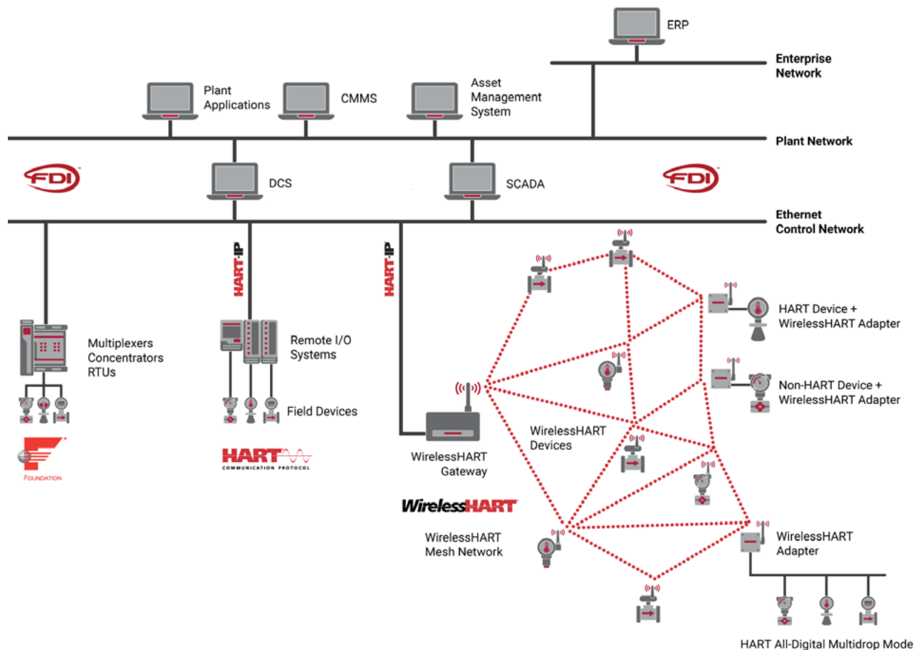
Figure 2: WirelessHART adapters can be used to free stranded data from 4-20mA HART instruments, and to connect non-HART 4-20mA instruments to WirelessHART networks.
