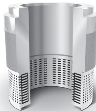
Figure 5. When extreme noise reduction is required, solutions are available that can be used to achieve noise reduction levels as high as 40 dB.
