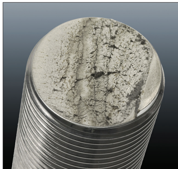
Figure 2. Control valve noise above 110 dBA external to the pipe can fatigue bolts and ultimately crack control valve stems and shafts. For this reason, sound levels should be kept below this threshold.
